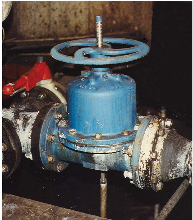
Straightway Valve on Abrasive Slurry Service
