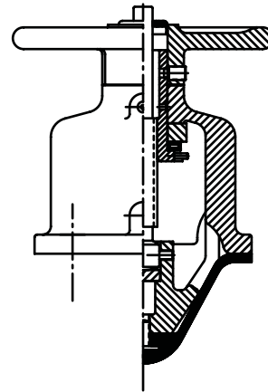
902 Bonnet Assembly
