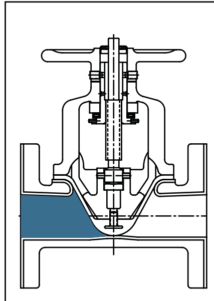
VALVE CLOSED
