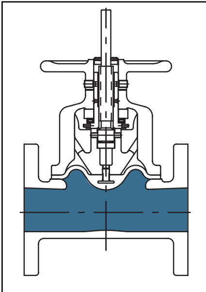
VALVE OPEN
