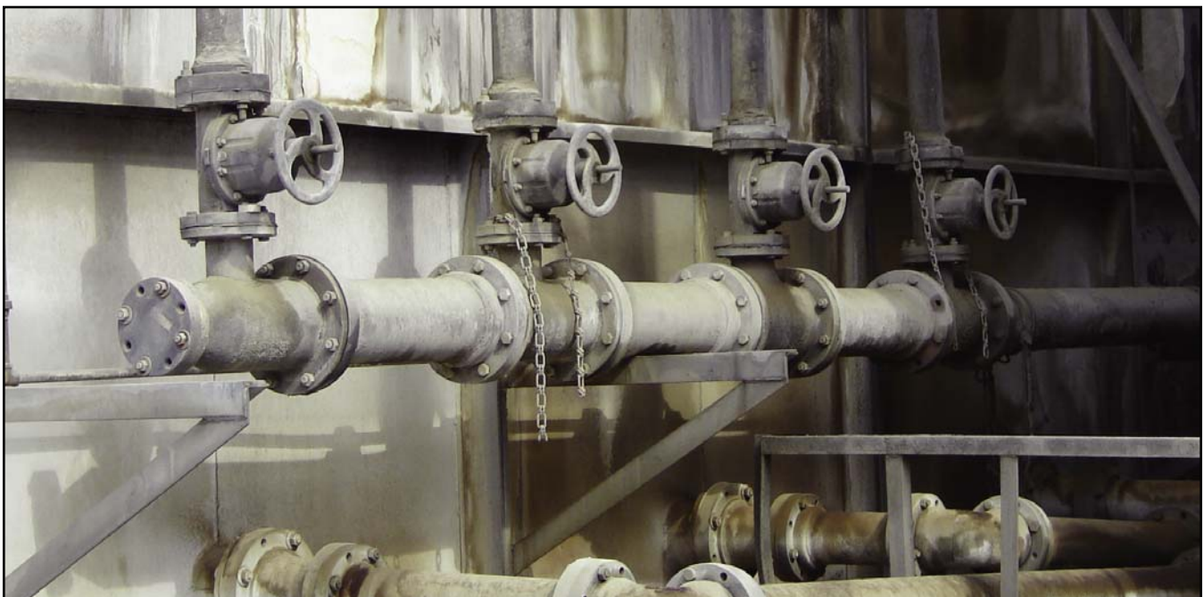
Straightway rubber lined valves in phosphoric acid service.
