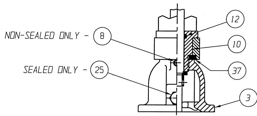
00.75 & 01.00 STEEL BONNET YOKE MOUNTED
